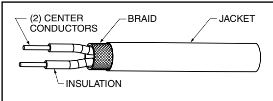
Cable Illustration - Differential Twinax Contact
