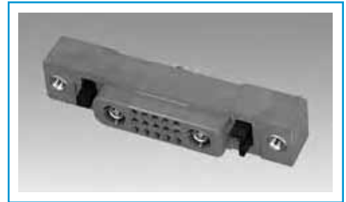
Low Mating Force PCB Connector with combination of signal Brush contacts and Coax contacts
